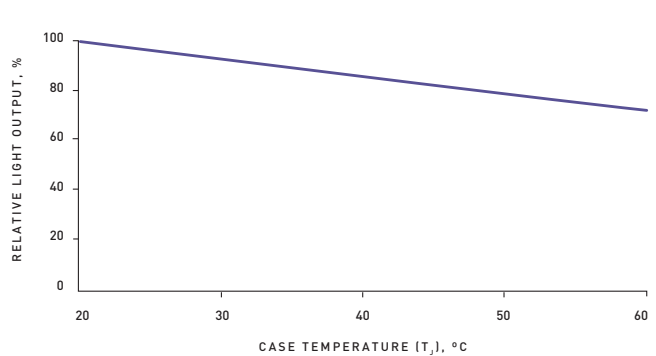
LIGHT OUTPUT OVER TEMPERATURE
