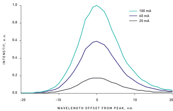
SPECTRUM VS. CURRENT
