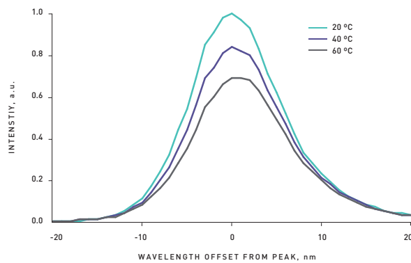
SPECTRUM VS. TEMPERATURE
