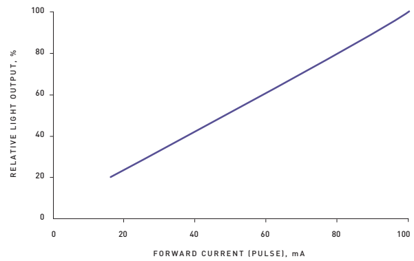
LIGHT OUTPUT OVER CURRENT
