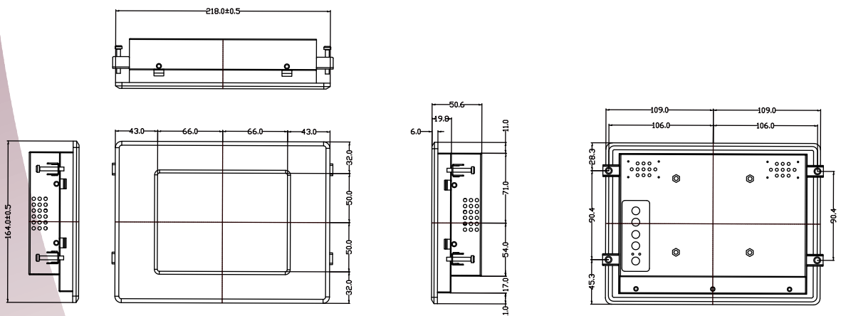
CUT OUT DIMENSION(191x142mm) UNIT:mm
