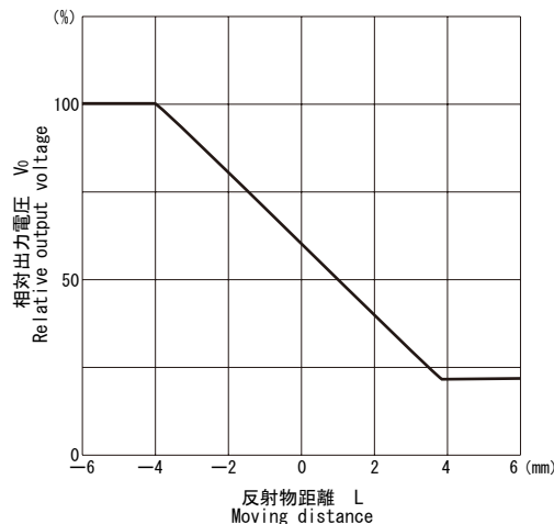
*2 Method of measuring position detection characteristic (Y)
