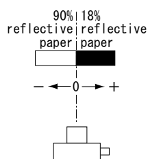
*2 Method of measuring position detection characteristic (Y)
